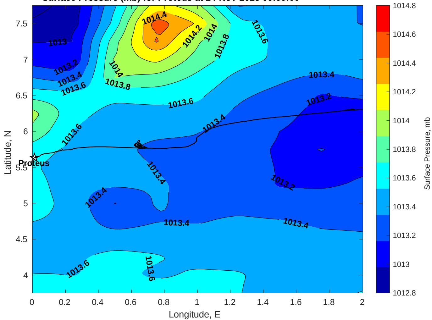
Surface Pressure (mb) for Proteus at 14-Nov-2025 00:00:00
