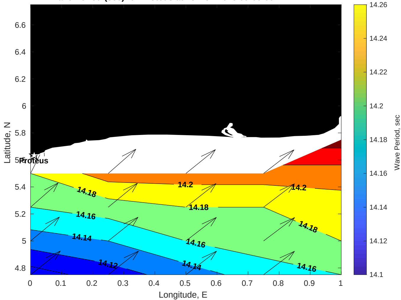
Wave Period (sec) for Proteus at 13-Nov-2025 09:00:00
