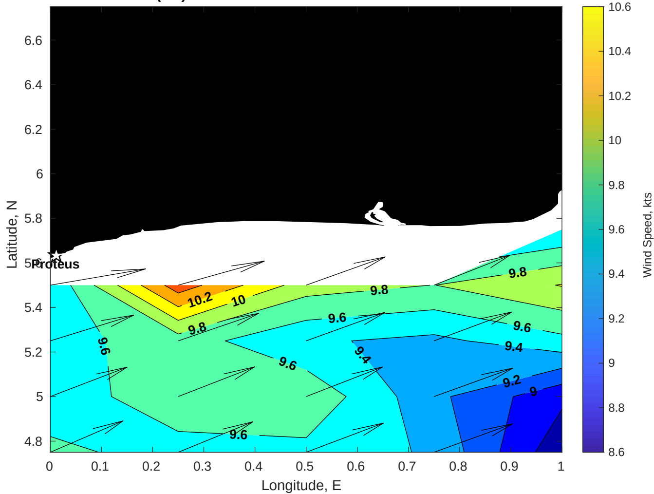
Winds (kts) for Proteus at 13-Nov-2025 09:00:00
