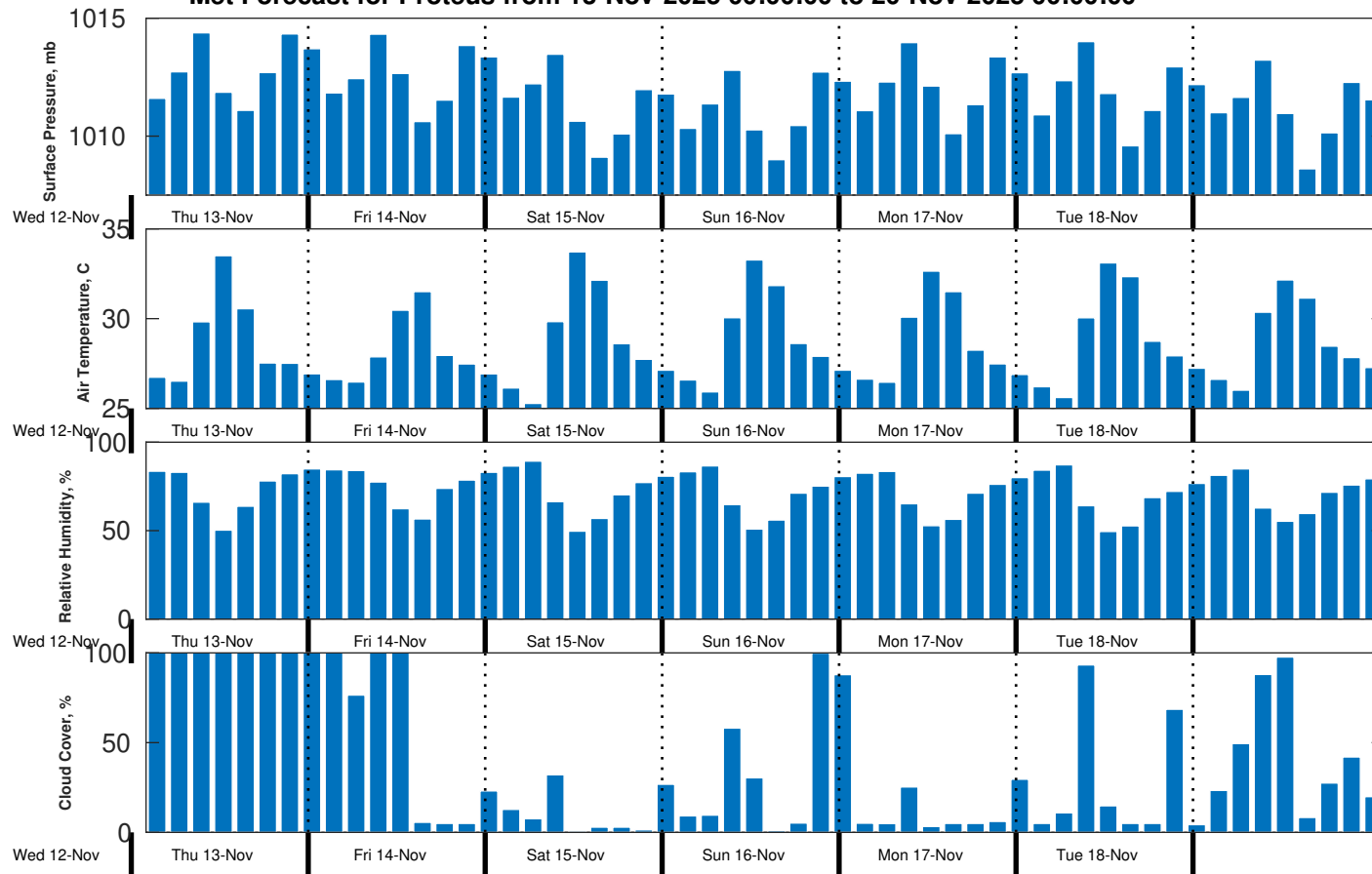
Met Forecast for Proteus from 13-Nov-2025 00:00:00 to 20-Nov-2025 00:00:00
