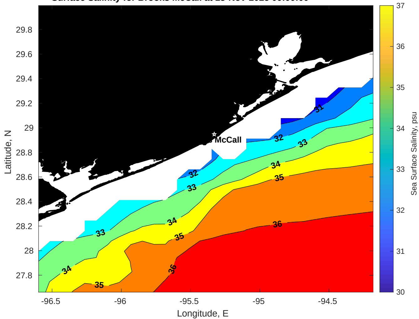
Surface Salinity for Brooks McCall at 13-Nov-2025 00:00:00
