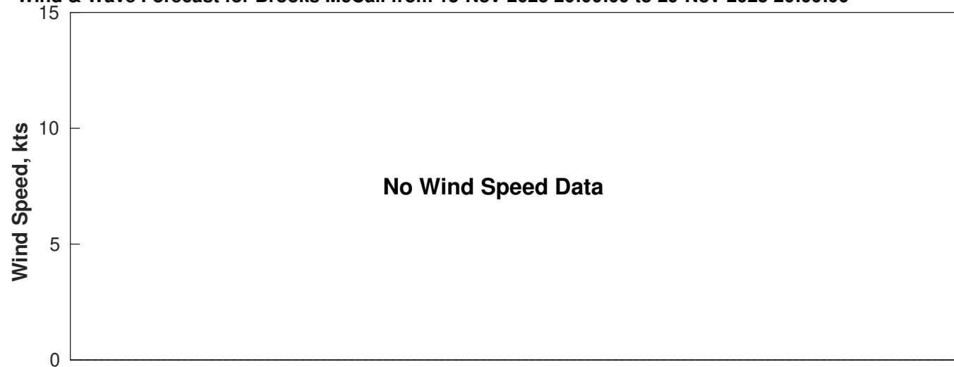
Wind & Wave Forecast for Brooks McCall from 13-Nov-2025 20:00:00 to 29-Nov-2025 20:00:00
