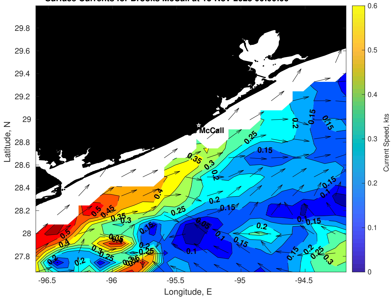
Surface Currents for Brooks McCall at 13-Nov-2025 00:00:00
