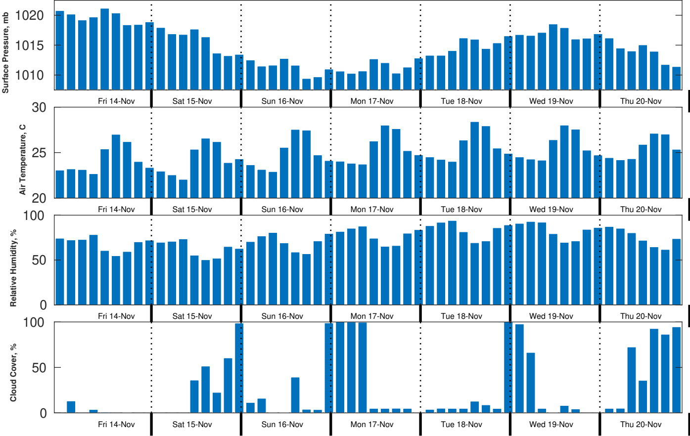
Met Forecast for Brooks McCall from 14-Nov-2025 00:00:00 to 21-Nov-2025 00:00:00
