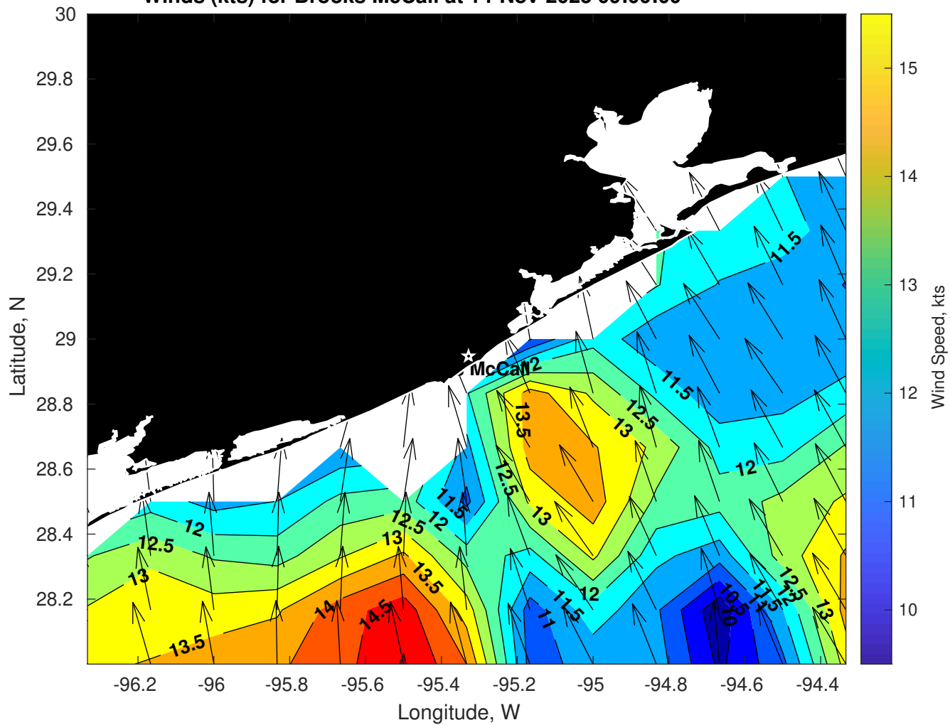
Winds (kts) for Brooks McCall at 14-Nov-2025 09:00:00
