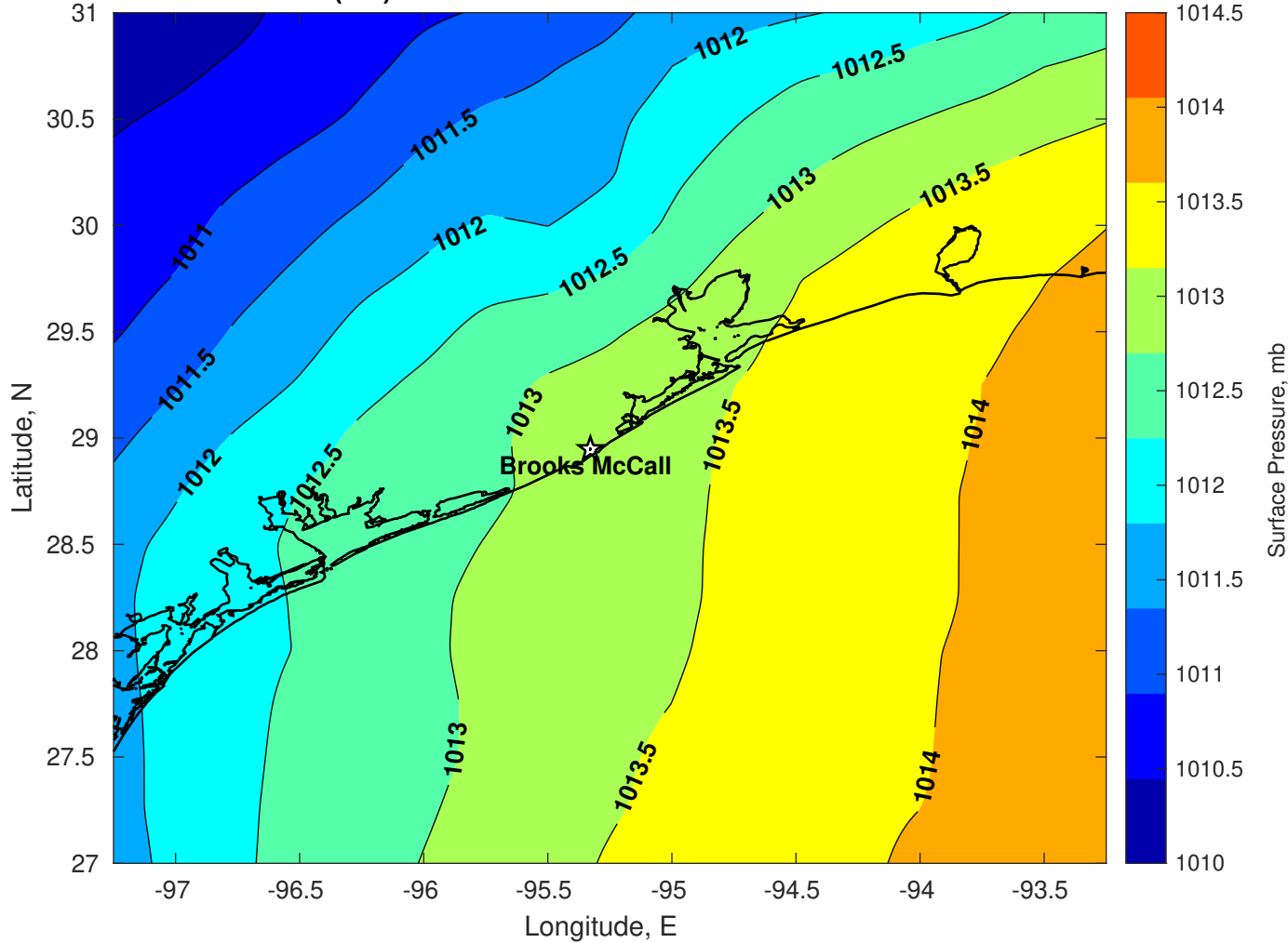
Surface Pressure (mb) for Brooks McCall at 16-Nov-2025 00:00:00
