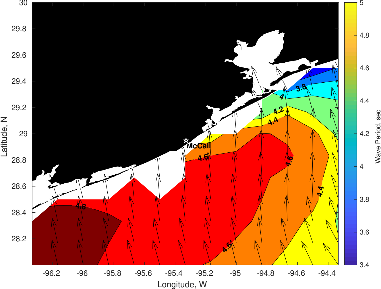
Wave Period (sec) for Brooks McCall at 14-Nov-2025 09:00:00
