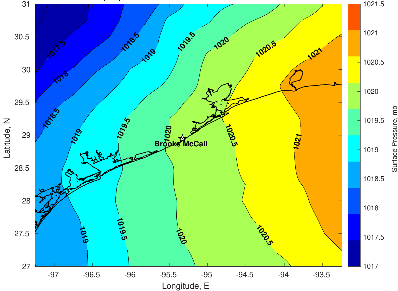
Surface Pressure (mb) for Brooks McCall at 14-Nov-2025 00:00:00
