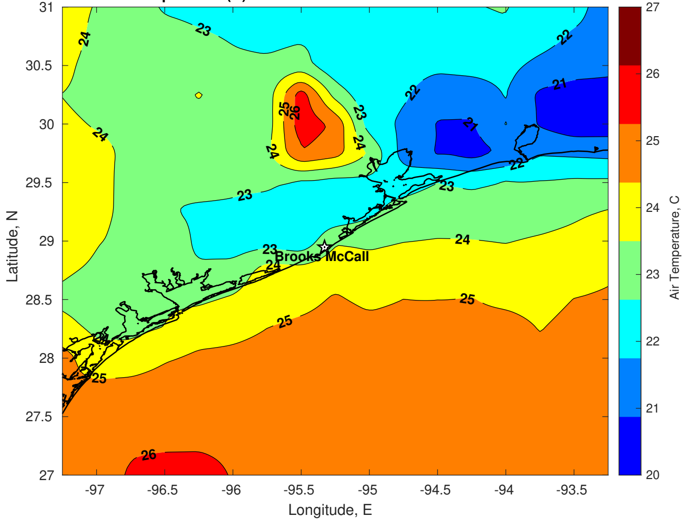
Air Temperature (C) for Brooks McCall at 14-Nov-2025
