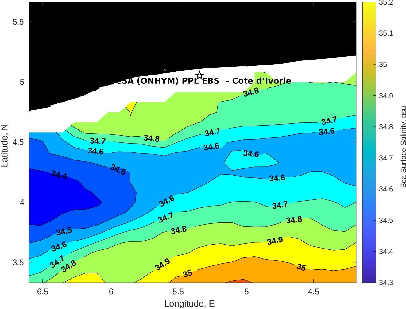
Surface Salinity for CSA (ONHYM) PPL EBS - Cote d'Ivoire at 13-Nov-2025 00:00:00
