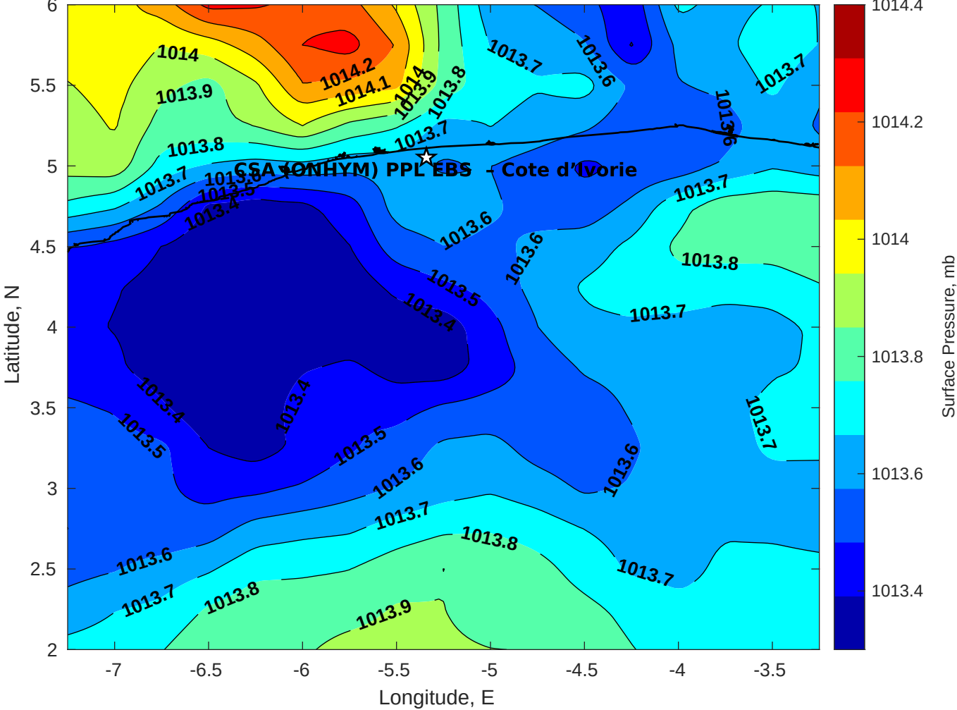
Surface Pressure (mb) for CSA (ONHYM) PPL EBS - Cote d'Ivoire at 15-Nov-2025 00:00:00
