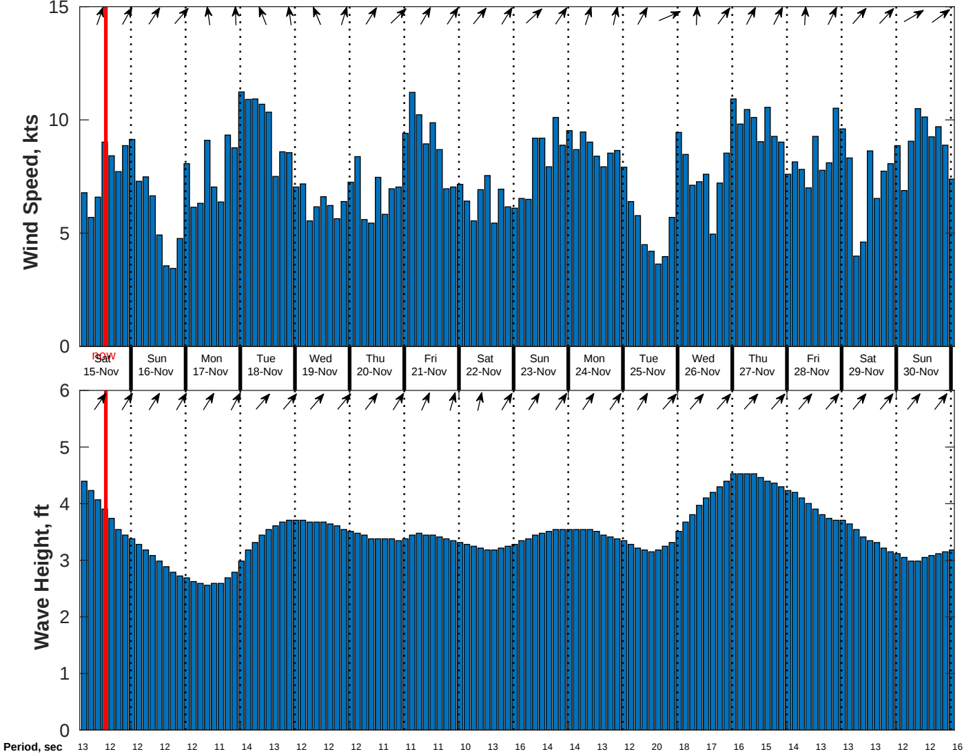
Wind & Wave Forecast for CSA (ONHYM) PPL EBS - Ghana from 14-Nov-2025 02:00:00 to 30-Nov-2025 02:00:00
