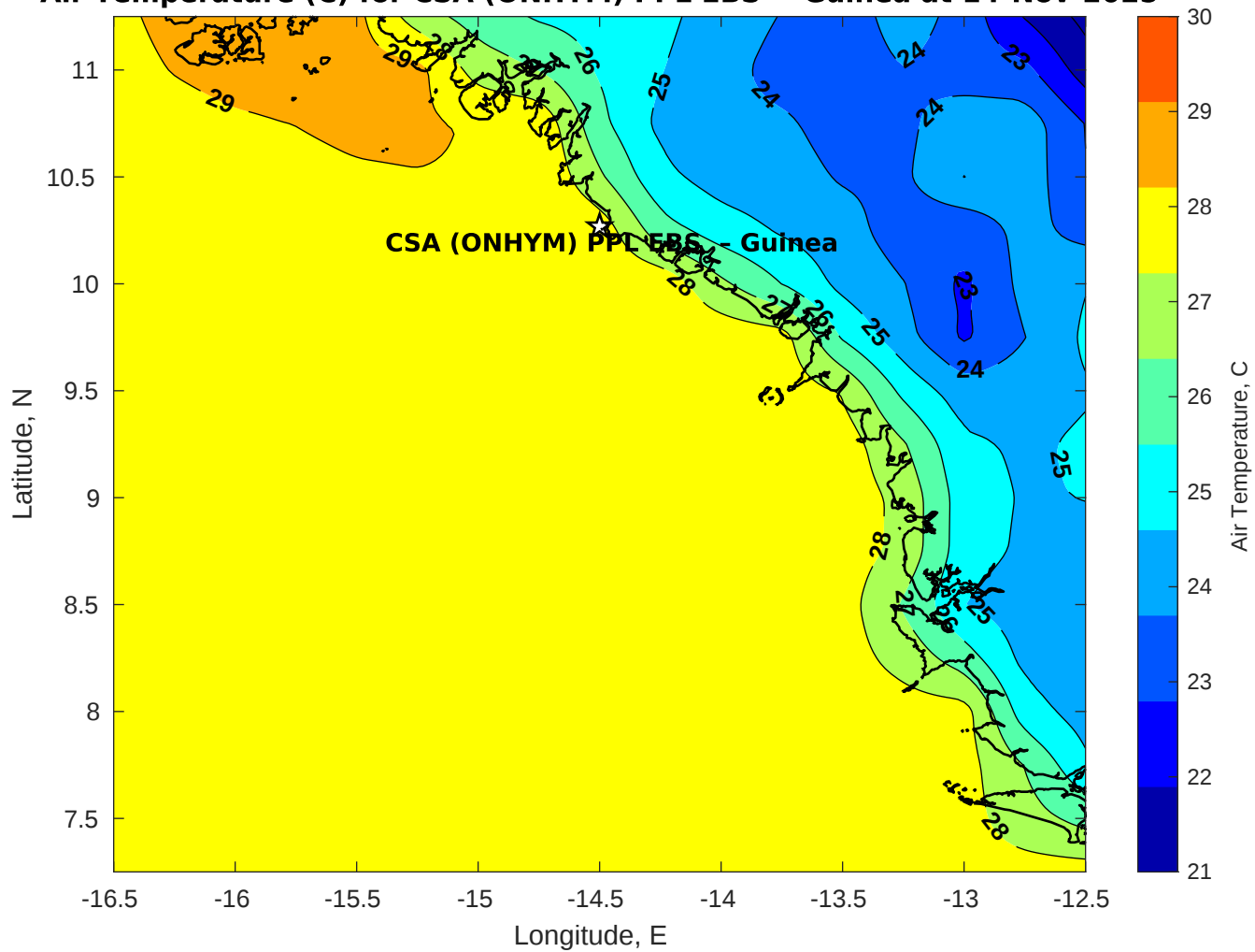
Air Temperature (C) for CSA (ONHYM) PPL EBS - Guinea at 14-Nov-2025
