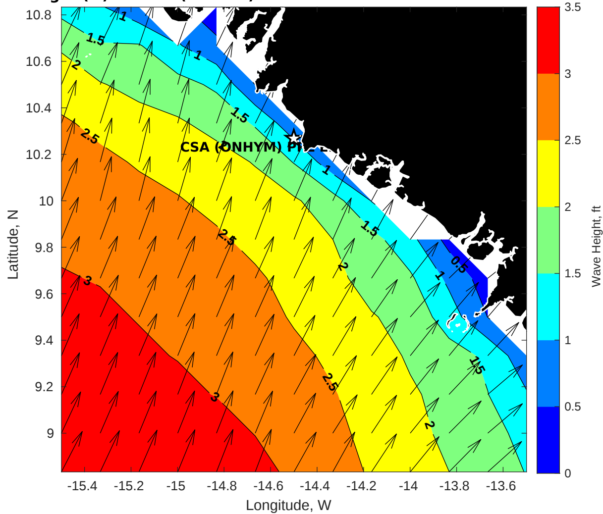
Wave Height (ft) for CSA (ONHYM) PPL EBS - Guinea at 14-Nov-2025 09:00:00
