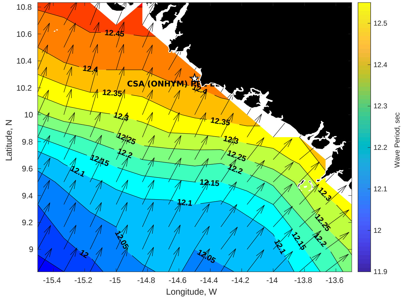
Wave Period (sec) for CSA (ONHYM) PPL EBS - Guinea at 14-Nov-2025 09:00:00
