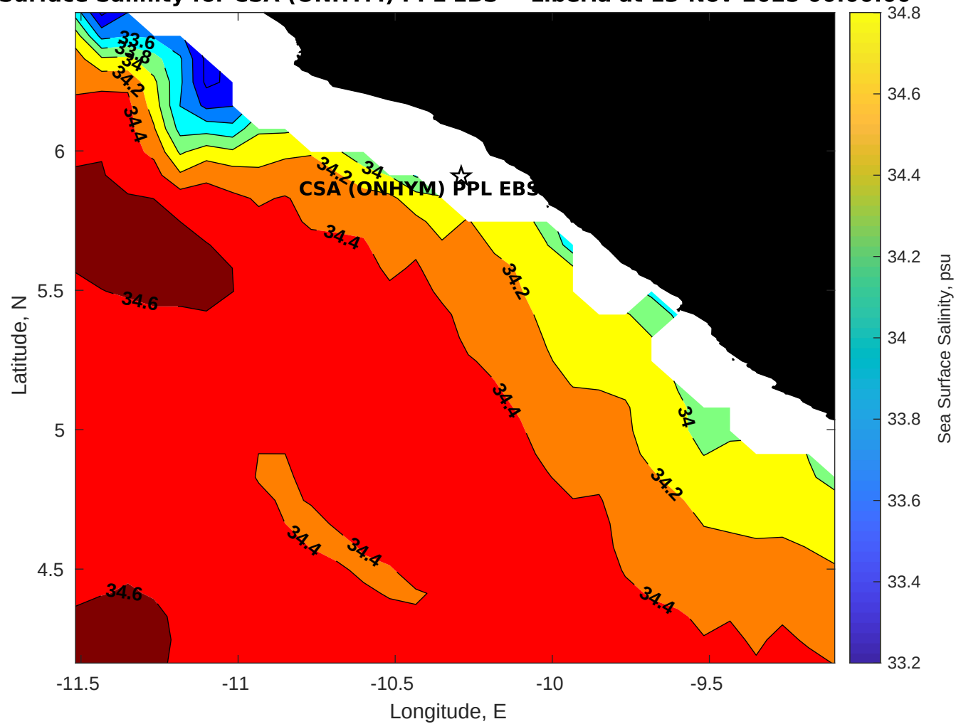
Surface Salinity for CSA (ONHYM) PPL EBS - Liberia at 13-Nov-2025 00:00:00
