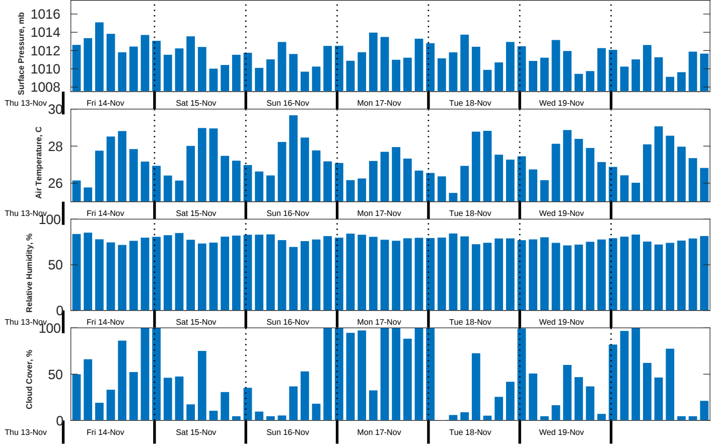
Met Forecast for CSA (ONHYM) PPL EBS - Liberia from 14-Nov-2025 00:00:00 to 21-Nov-2025 00:00:00
