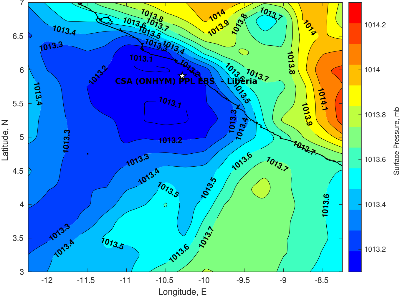
Surface Pressure (mb) for CSA (ONHYM) PPL EBS - Liberia at 15-Nov-2025 00:00:00
