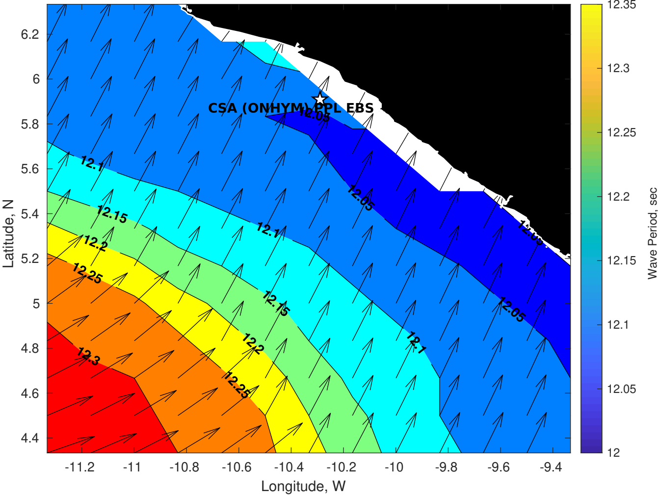
Wave Period (sec) for CSA (ONHYM) PPL EBS - Liberia at 14-Nov-2025 09:00:00
