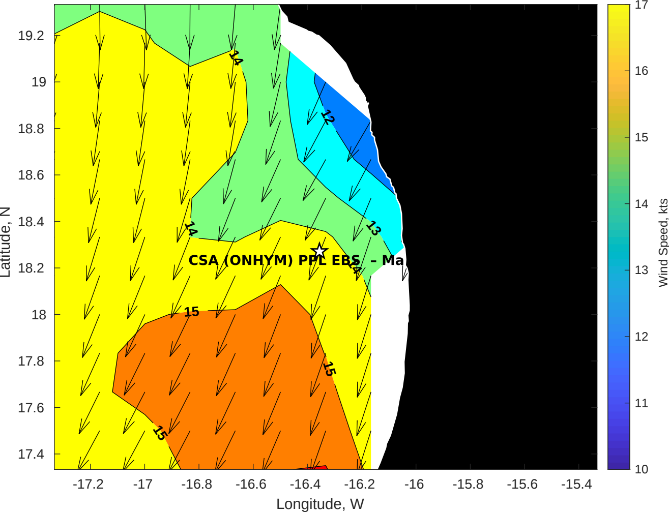
Winds (kts) for CSA (ONHYM) PPL EBS - Mauritania at 14-Nov-2025 09:00:00
