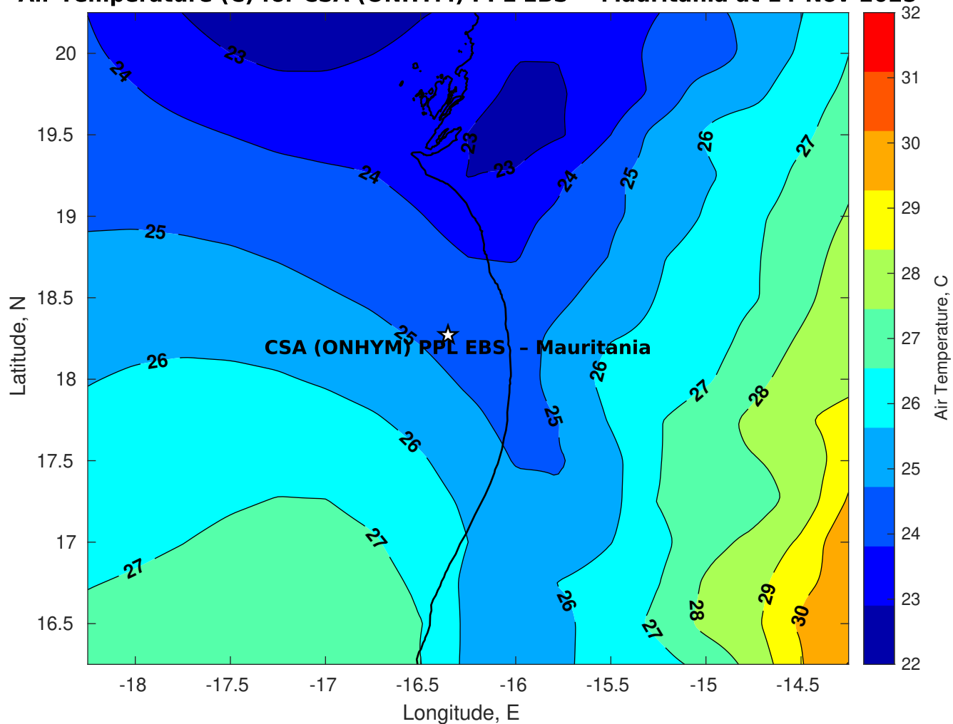
Air Temperature (C) for CSA (ONHYM) PPL EBS - Mauritania at 14-Nov-2025
