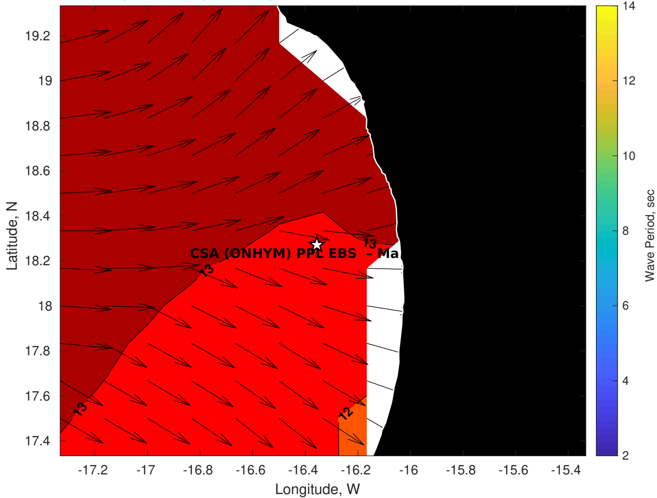
Wave Period (sec) for CSA (ONHYM) PPL EBS - Mauritania at 14-Nov-2025 09:00:00
