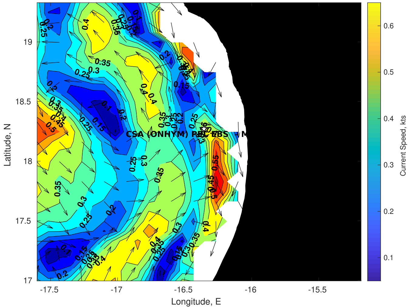
Surface Currents for CSA (ONHYM) PPL EBS - Mauritania at 13-Nov-2025 00:00:00
