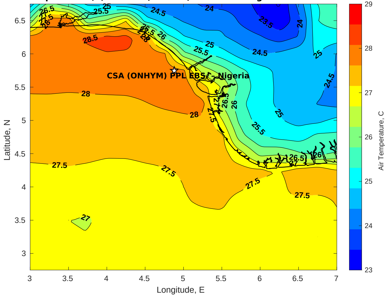
Air Temperature (C) for CSA (ONHYM) PPL EBS - Nigeria at 14-Nov-2025
