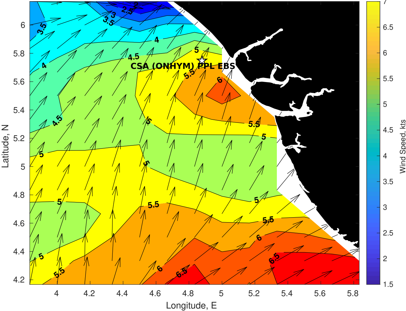
Winds (kts) for CSA (ONHYM) PPL EBS - Nigeria at 14-Nov-2025 09:00:00
