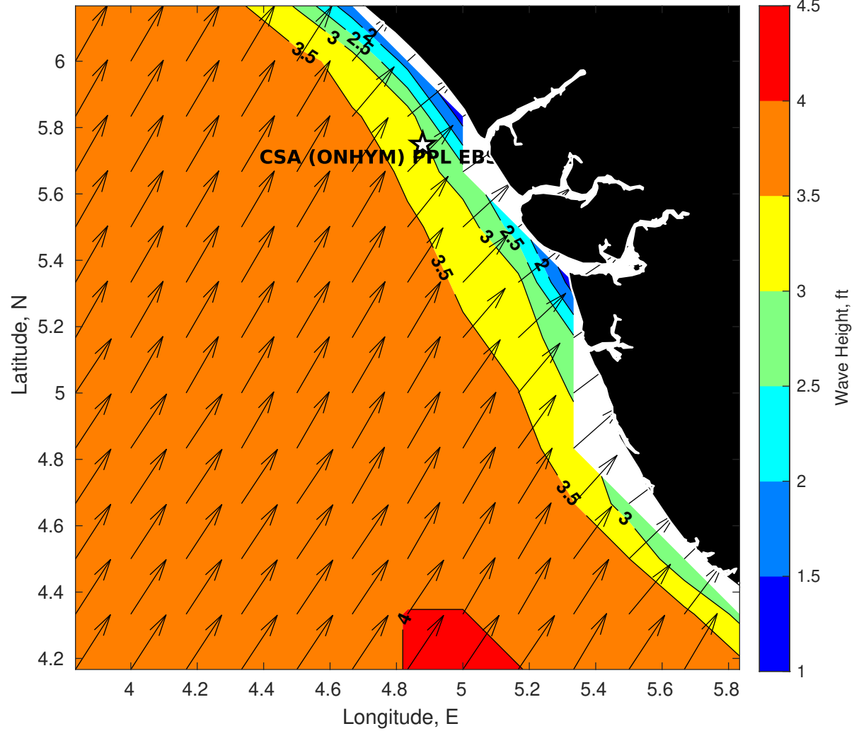
Wave Height (ft) for CSA (ONHYM) PPL EBS - Nigeria at 14-Nov-2025 09:00:00
