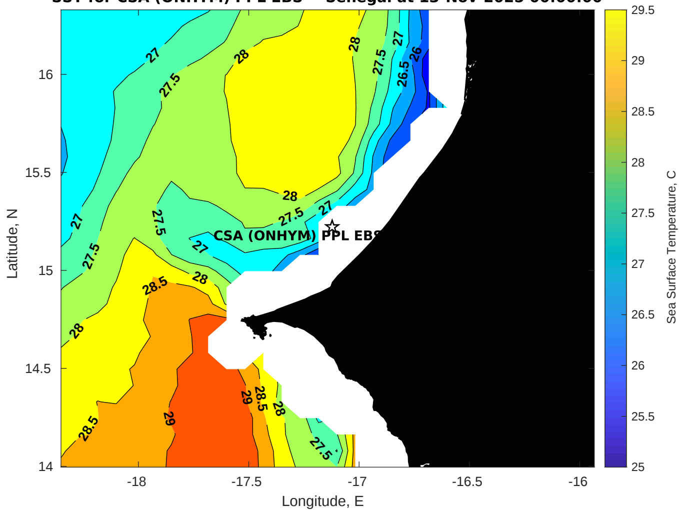
SST for CSA (ONHYM) PPL EBS - Senegal at 13-Nov-2025 00:00:00
