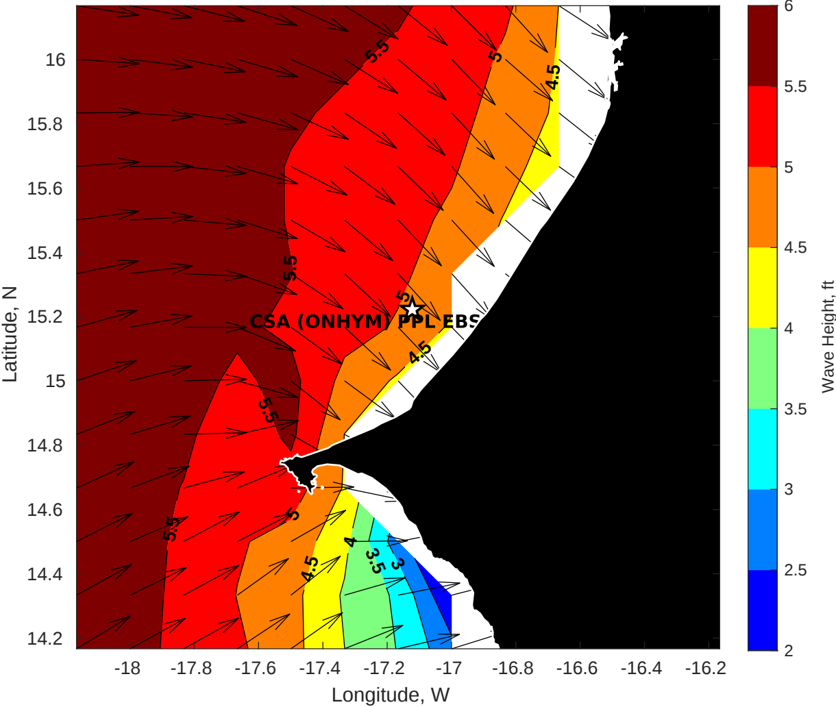
Wave Height (ft) for CSA (ONHYM) PPL EBS - Senegal at 14-Nov-2025 09:00:00
