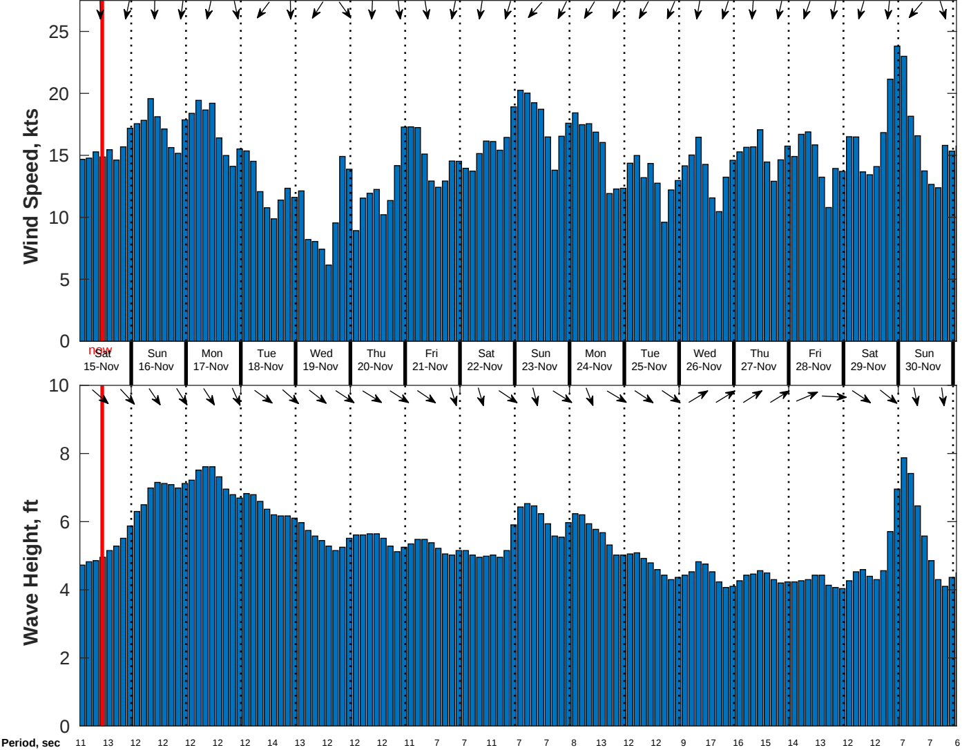
Wind & Wave Forecast for CSA (ONHYM) PPL EBS - Senegal from 14-Nov-2025 01:00:00 to 30-Nov-2025 01:00:00
