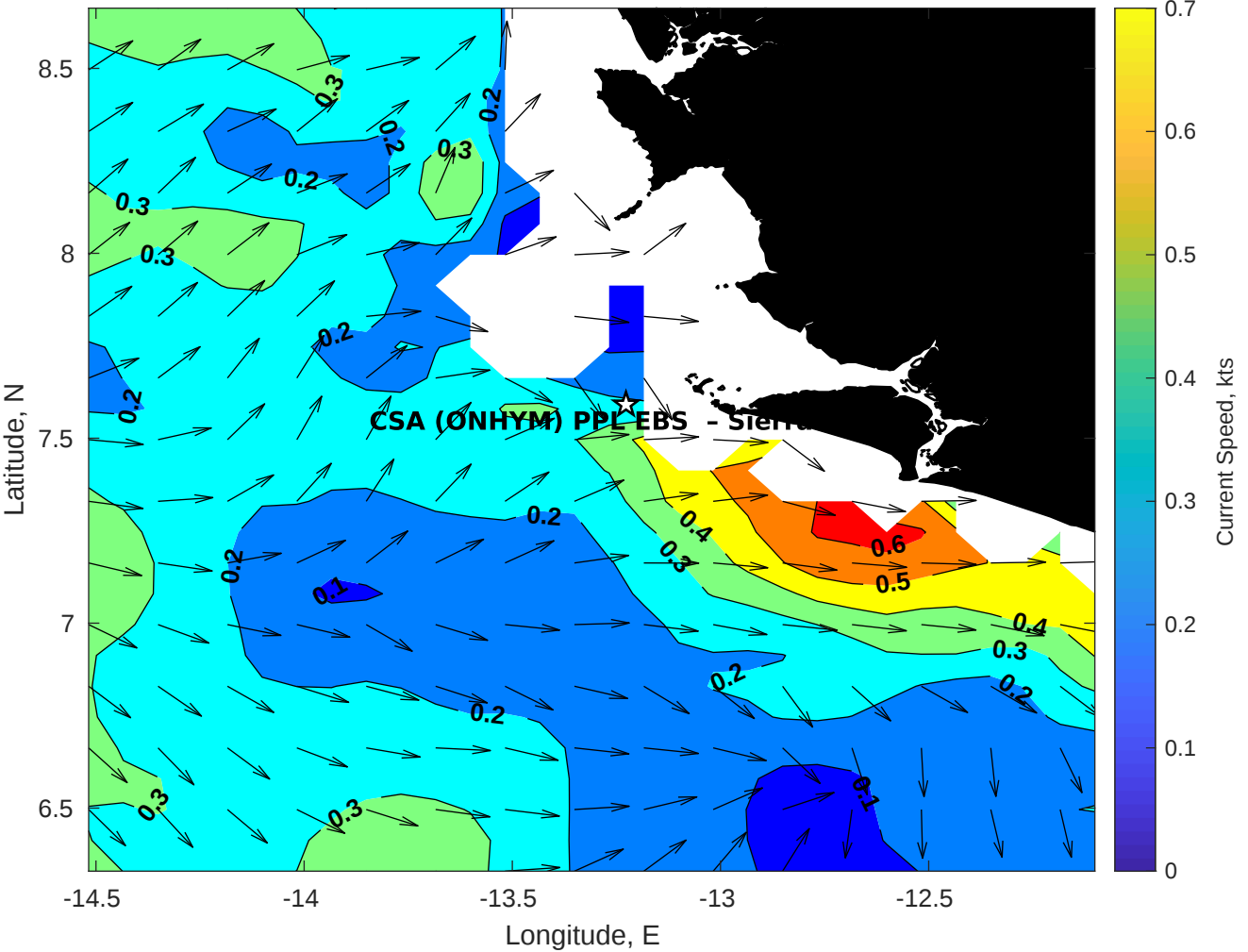
Surface Currents for CSA (ONHYM) PPL EBS - Sierra Leone at 13-Nov-2025 00:00:00
