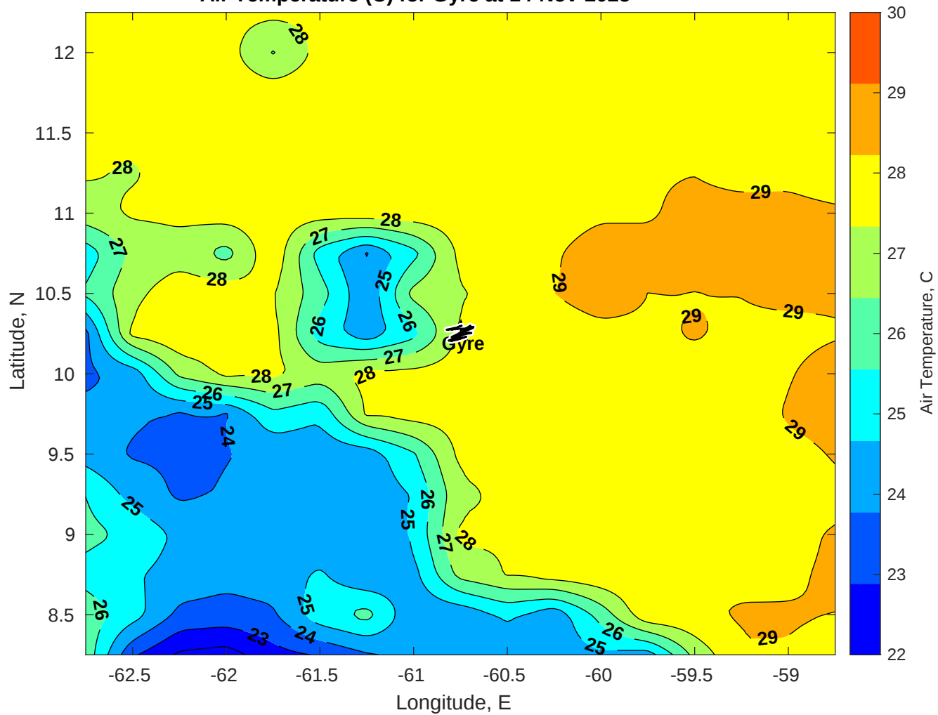
Air Temperature (C) for Gyre at 14-Nov-2025
