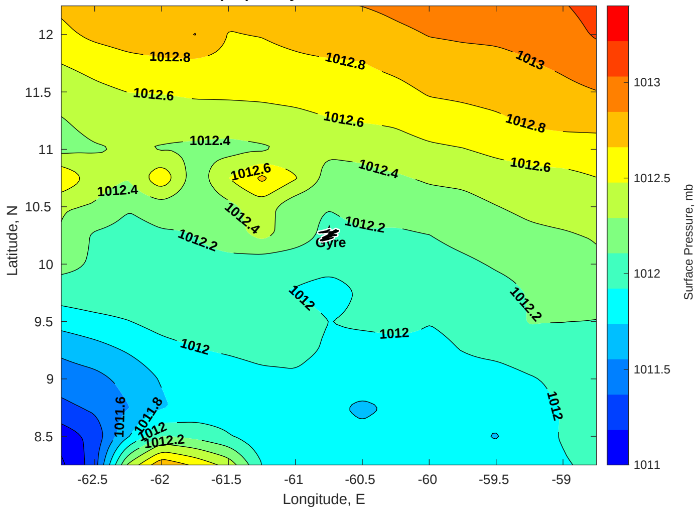
Surface Pressure (mb) for Gyre at 14-Nov-2025 00:00:00
