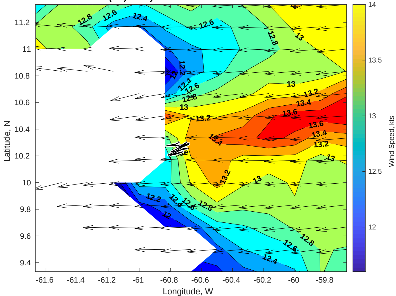
Winds (kts) for Gyre at 14-Nov-2025 09:00:00
