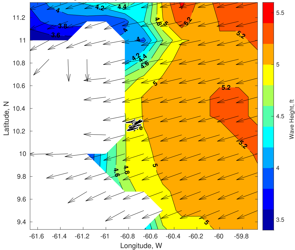
Wave Height (ft) for Gyre at 14-Nov-2025 09:00:00
