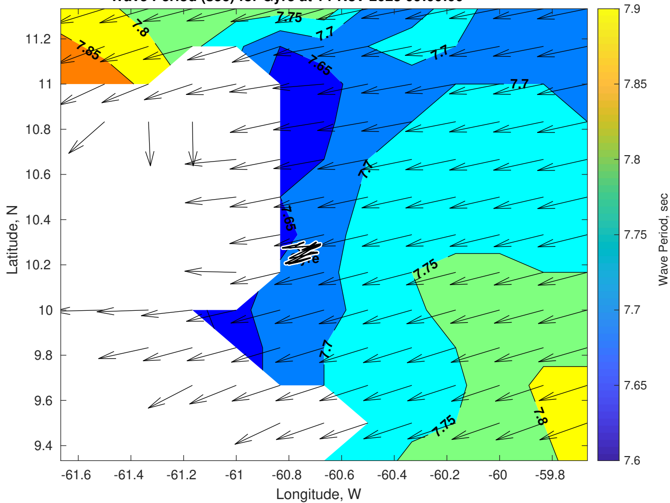
Wave Period (sec) for Gyre at 14-Nov-2025 09:00:00
