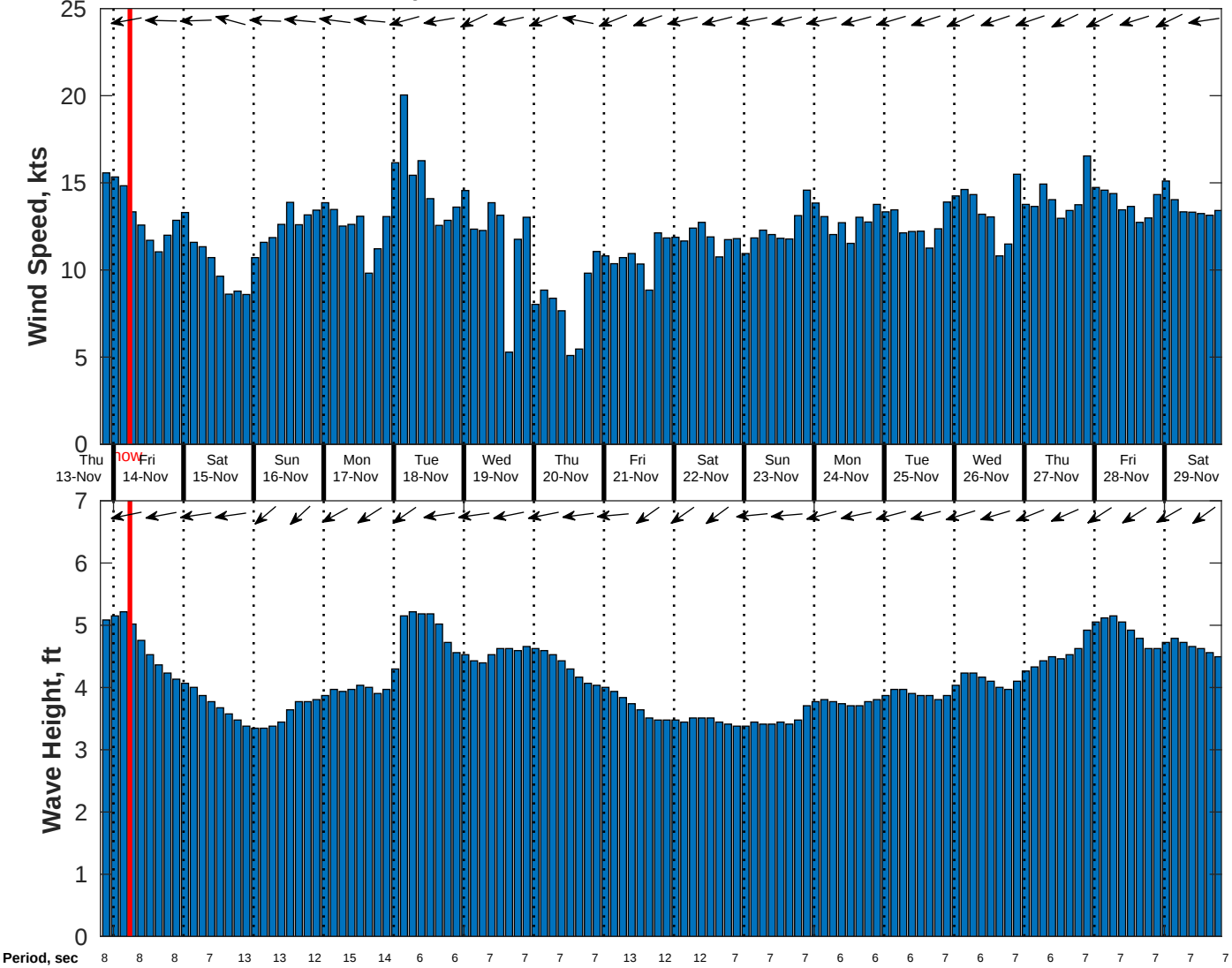
Wind & Wave Forecast for Gyre from 13-Nov-2025 20:00:00 to 29-Nov-2025 20:00:00
