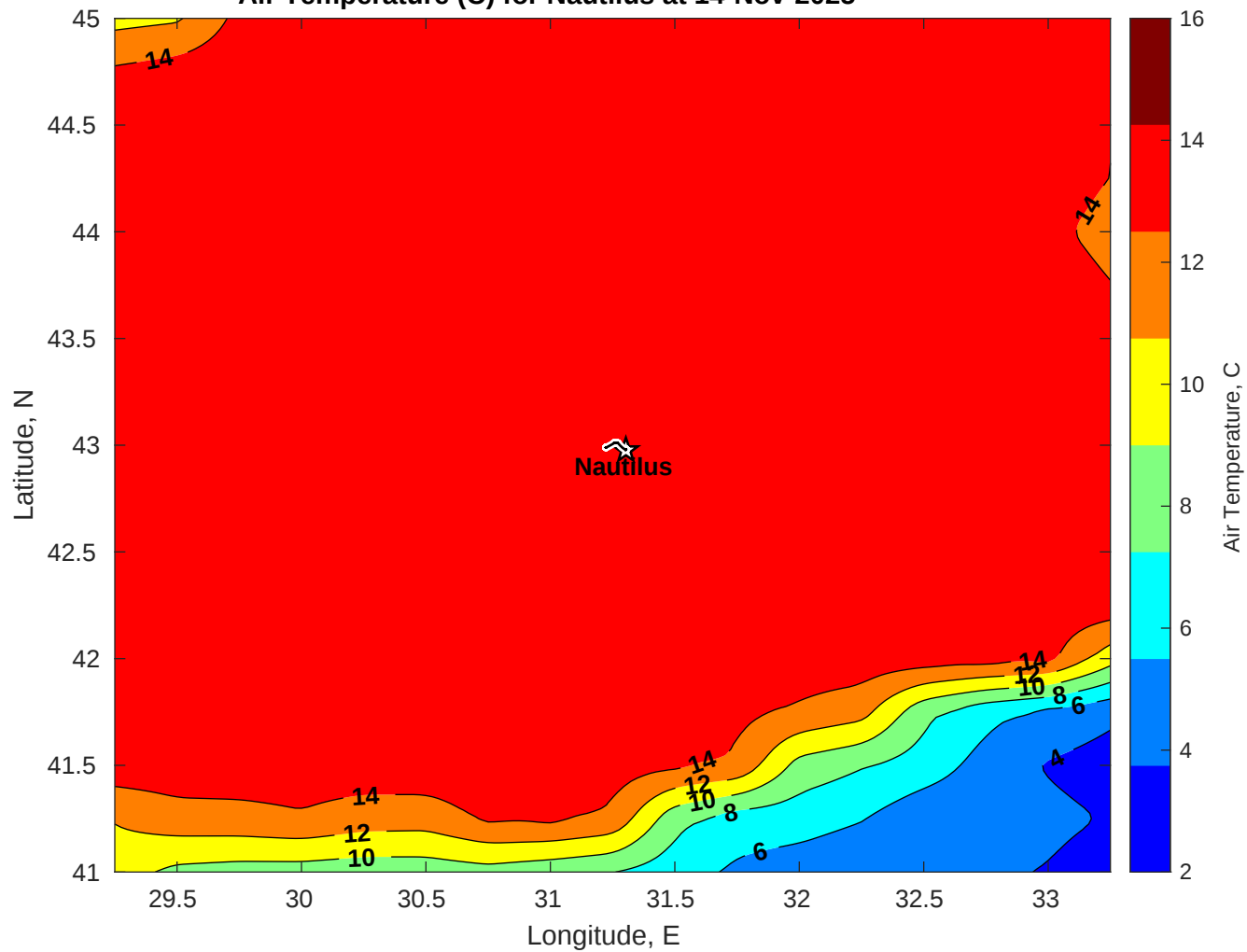
Air Temperature (C) for Nautilus at 14-Nov-2025
