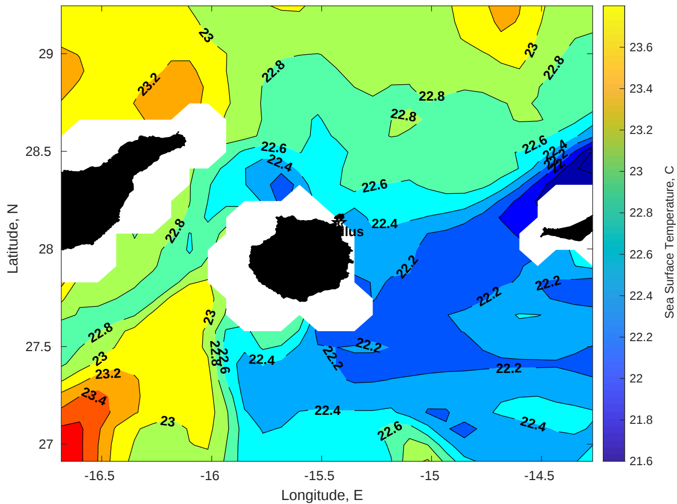
SST for Nautilus at 13-Nov-2025 00:00:00
