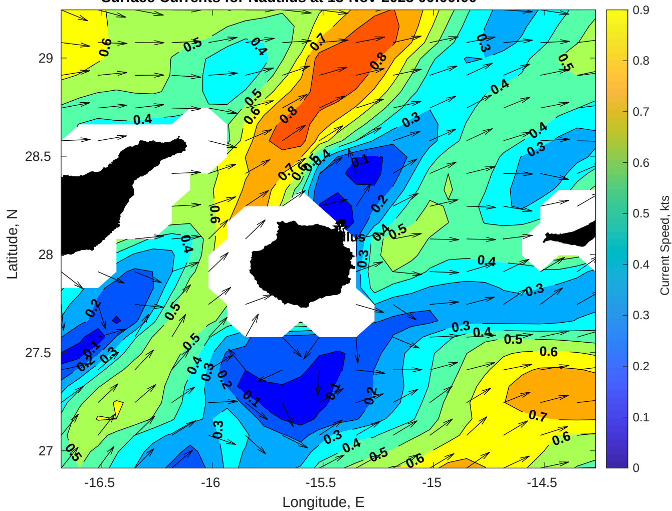
Surface Currents for Nautilus at 13-Nov-2025 00:00:00
