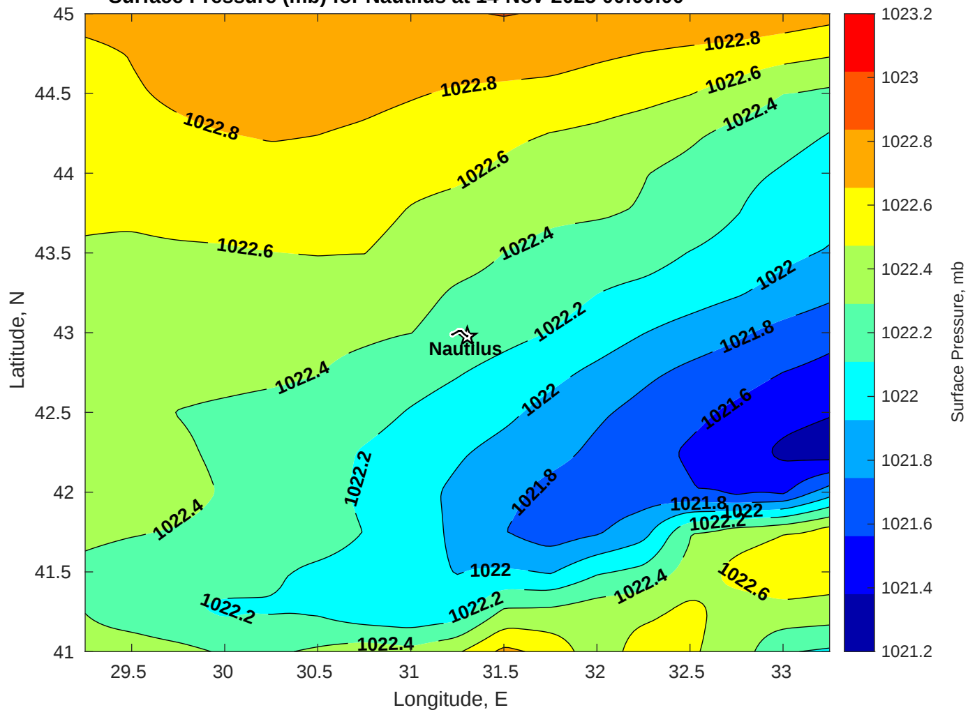
Surface Pressure (mb) for Nautilus at 14-Nov-2025 00:00:00
