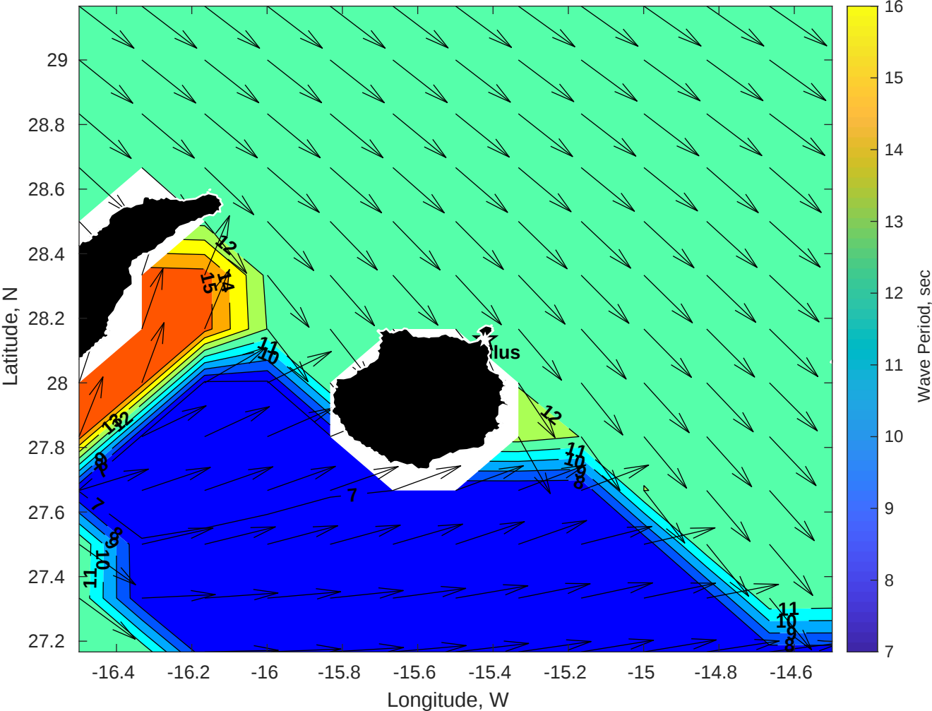
Wave Period (sec) for Nautilus at 13-Nov-2025 21:00:00
