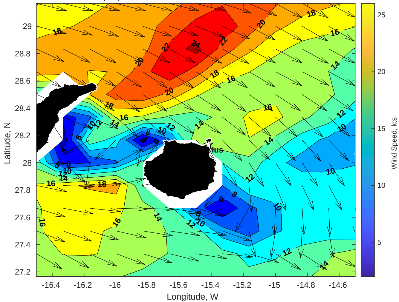
Winds (kts) for Nautilus at 13-Nov-2025 21:00:00
