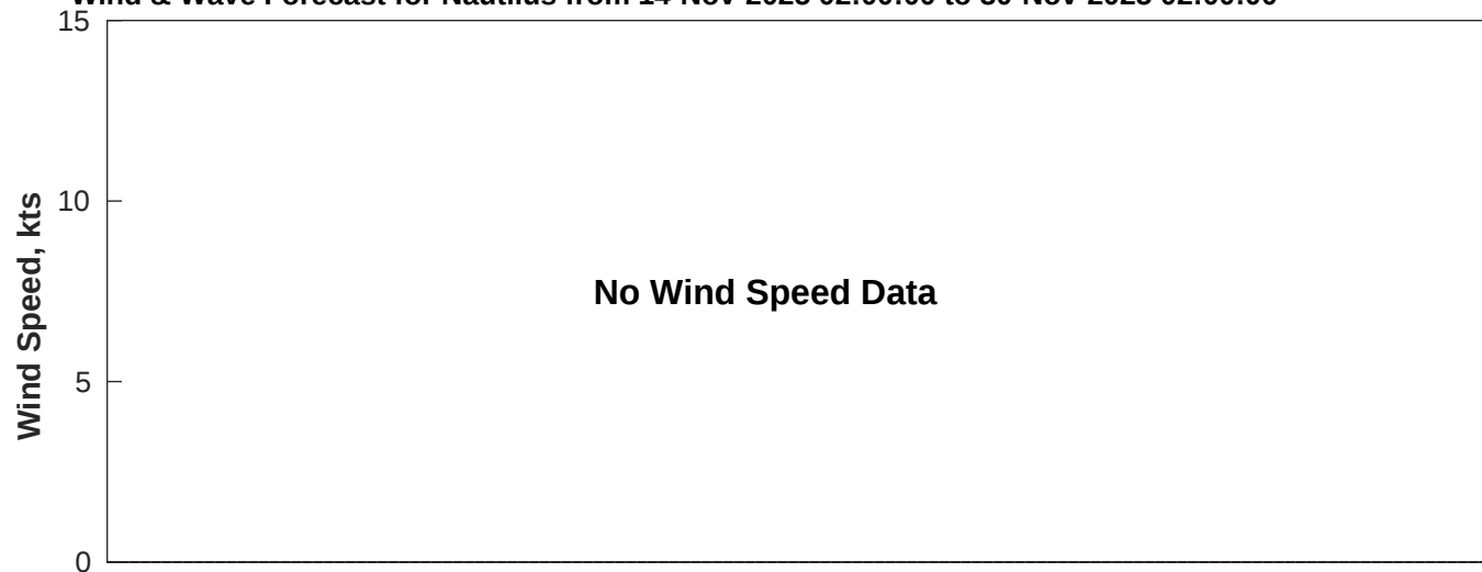
Wind & Wave Forecast for Nautilus from 14-Nov-2025 02:00:00 to 30-Nov-2025 02:00:00
