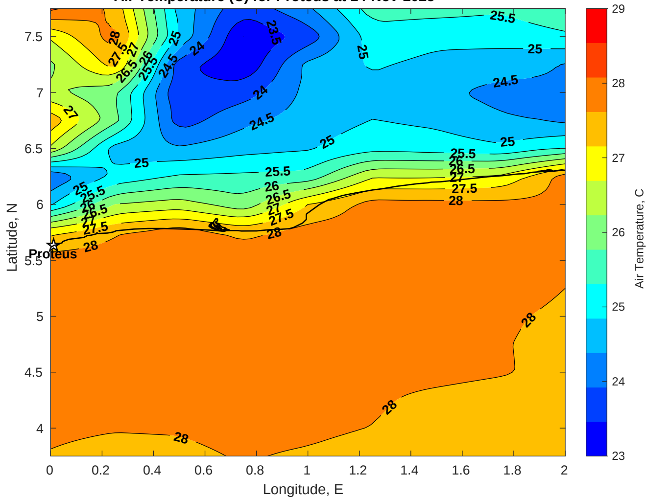
Air Temperature (C) for Proteus at 14-Nov-2025
