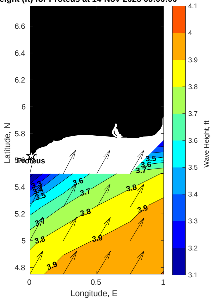
Wave Height (ft) for Proteus at 14-Nov-2025 09:00:00
