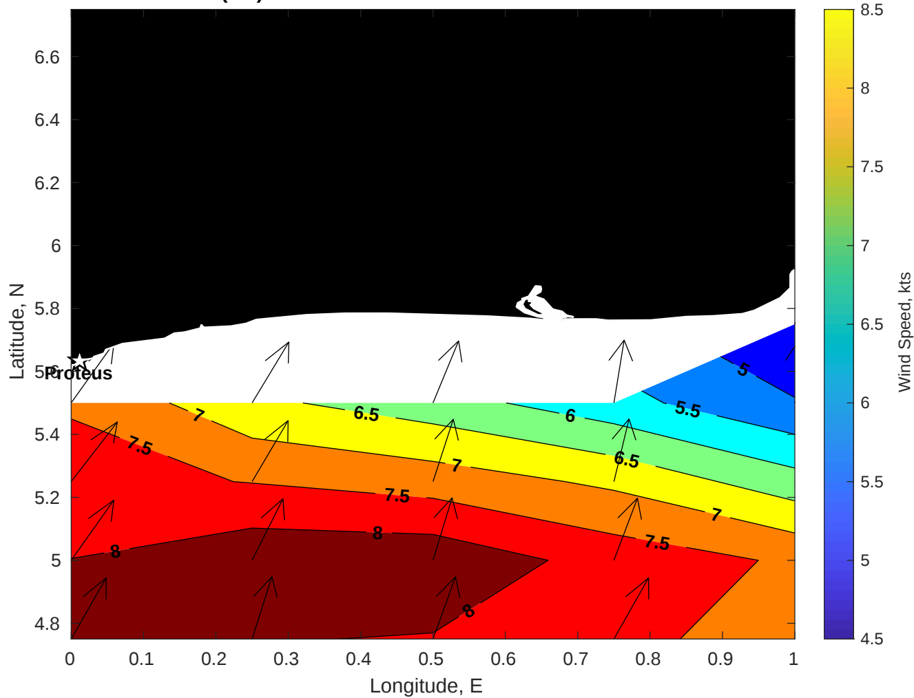
Winds (kts) for Proteus at 14-Nov-2025 09:00:00
