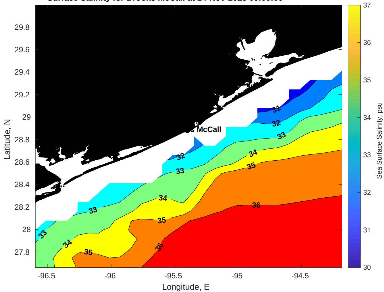
Surface Salinity for Brooks McCall at 14-Nov-2025 00:00:00
