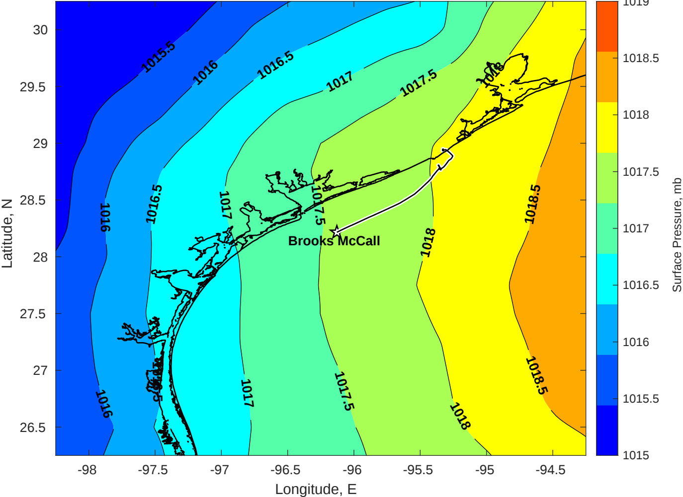
Surface Pressure (mb) for Brooks McCall at 15-Nov-2025 00:00:00
