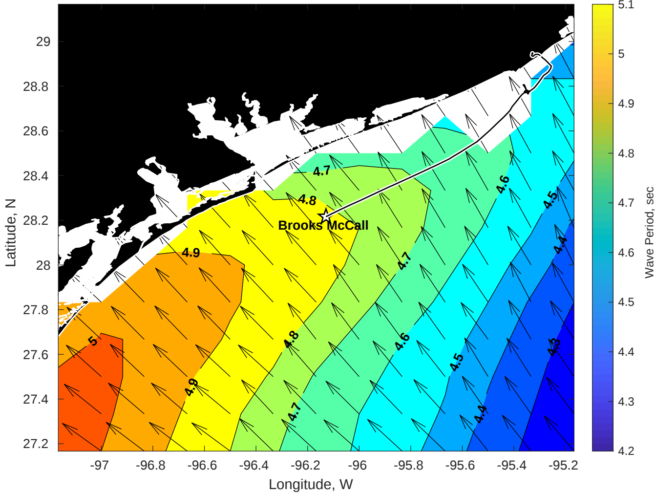
Wave Period (sec) for Brooks McCall at 15-Nov-2025 09:00:00
