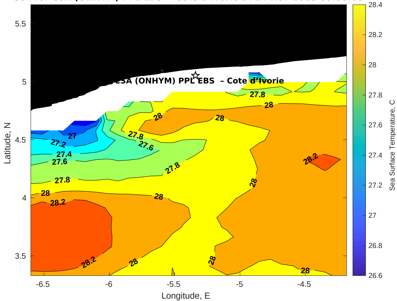
SST for CSA (ONHYM) PPL EBS - Cote d'Ivoire at 14-Nov-2025 00:00:00
