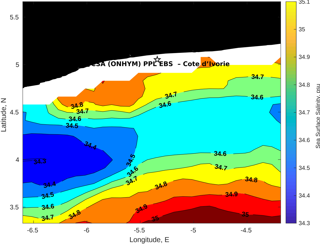
Surface Salinity for CSA (ONHYM) PPL EBS - Cote d'Ivoire at 14-Nov-2025 00:00:00
