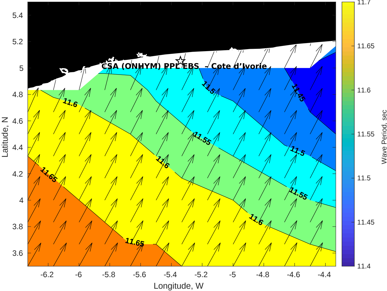
Wave Period (sec) for CSA (ONHYM) PPL EBS - Cote d'Ivoire at 15-Nov-2025 09:00:00
