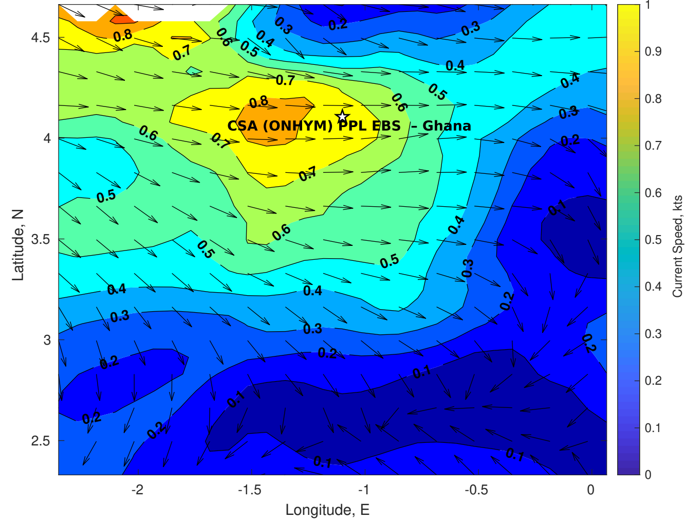
Surface Currents for CSA (ONHYM) PPL EBS - Ghana at 14-Nov-2025 00:00:00
