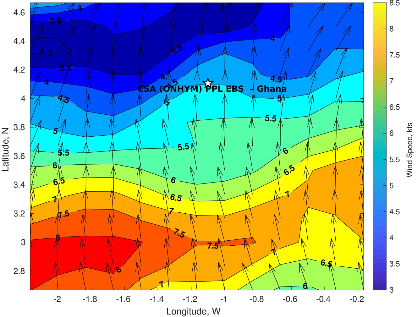
Winds (kts) for CSA (ONHYM) PPL EBS - Ghana at 15-Nov-2025 09:00:00
