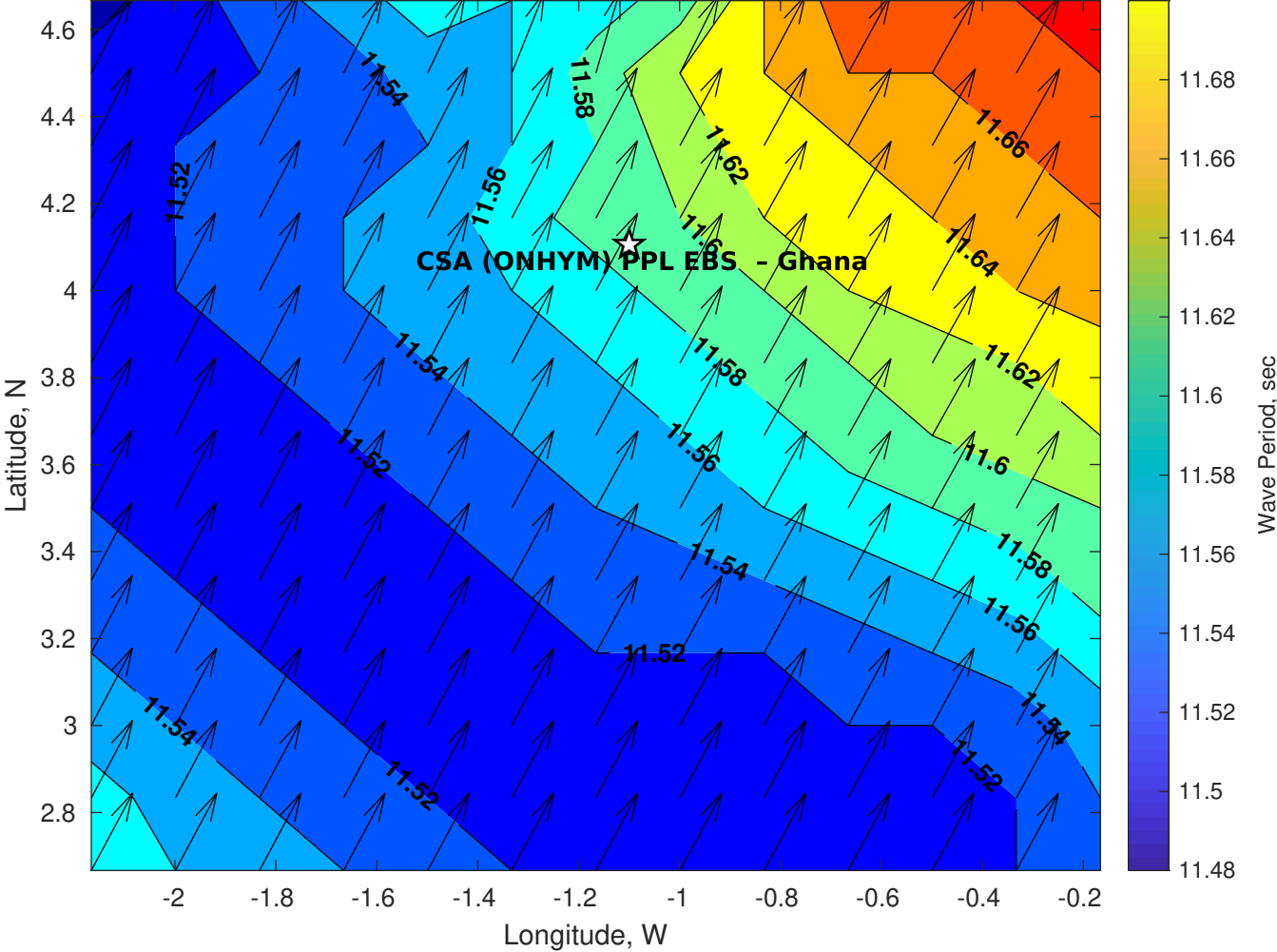
Wave Period (sec) for CSA (ONHYM) PPL EBS - Ghana at 15-Nov-2025 09:00:00
