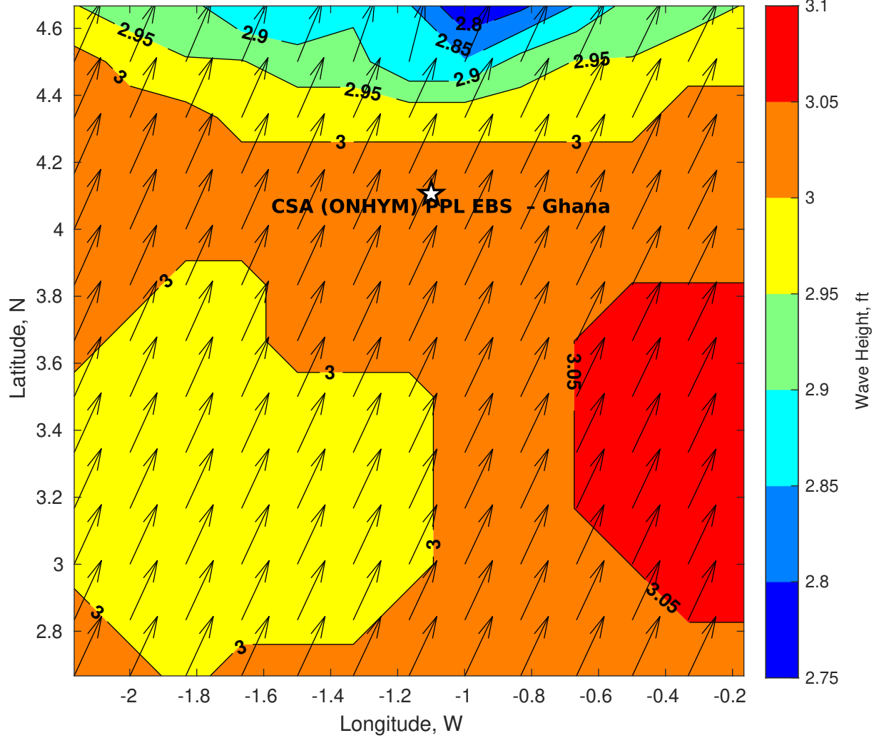
Wave Height (ft) for CSA (ONHYM) PPL EBS - Ghana at 15-Nov-2025 09:00:00
