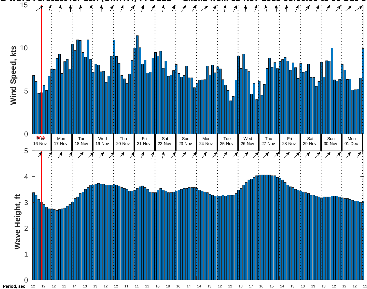
Wind & Wave Forecast for CSA (ONHYM) PPL EBS - Ghana from 15-Nov-2025 02:00:00 to 01-Dec-2025 02:00:00
