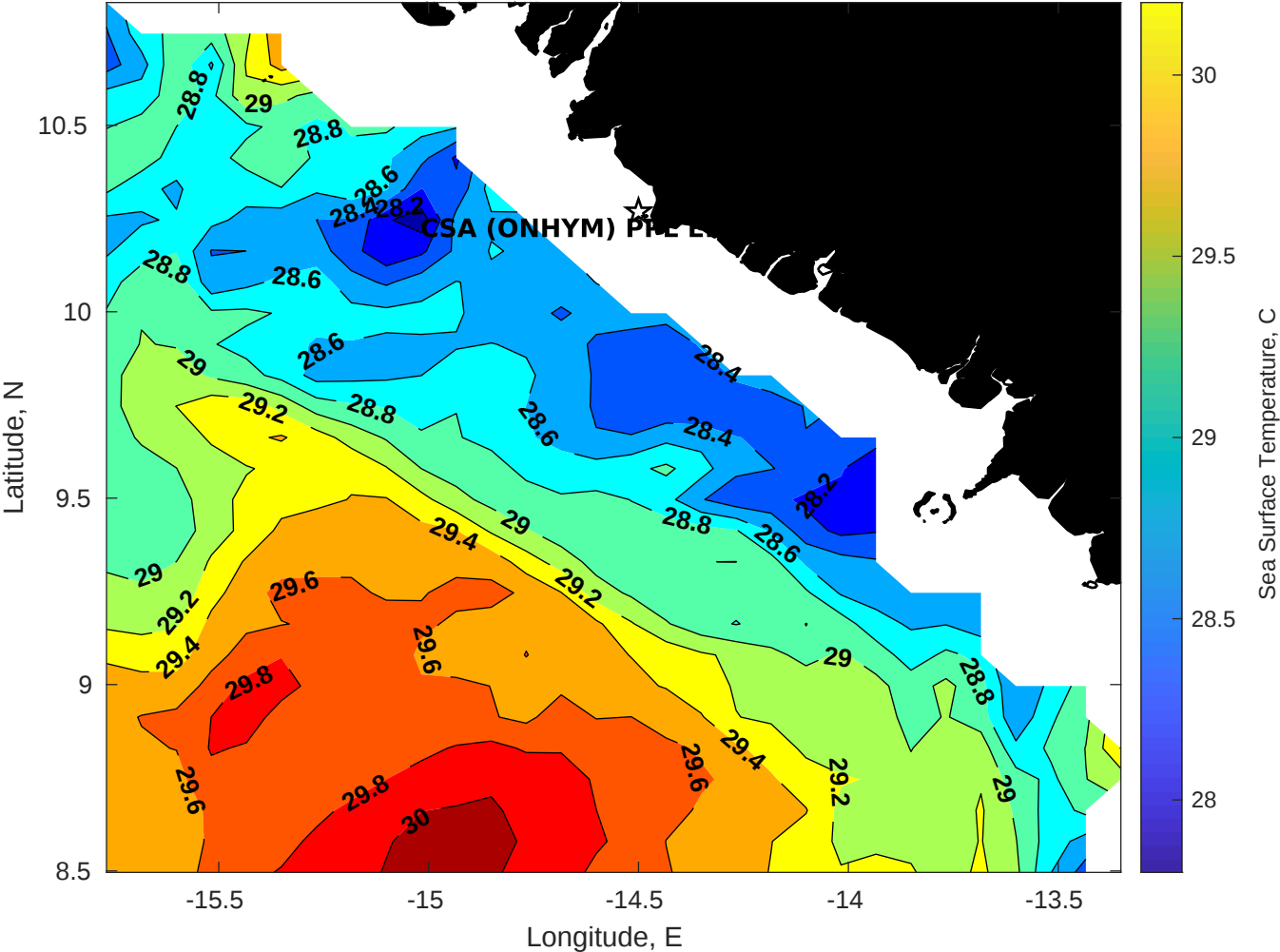
SST for CSA (ONHYM) PPL EBS - Guinea at 14-Nov-2025 00:00:00
