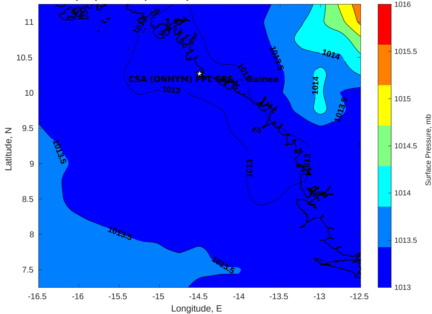
Surface Pressure (mb) for CSA (ONHYM) PPL EBS - Guinea at 15-Nov-2025 00:00:00
