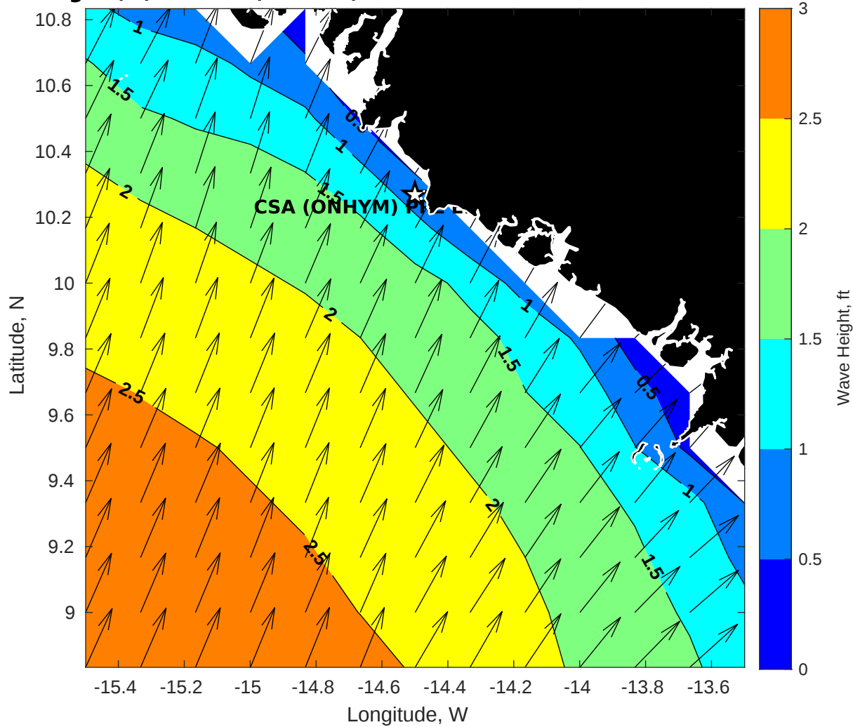
Wave Height (ft) for CSA (ONHYM) PPL EBS - Guinea at 15-Nov-2025 09:00:00
