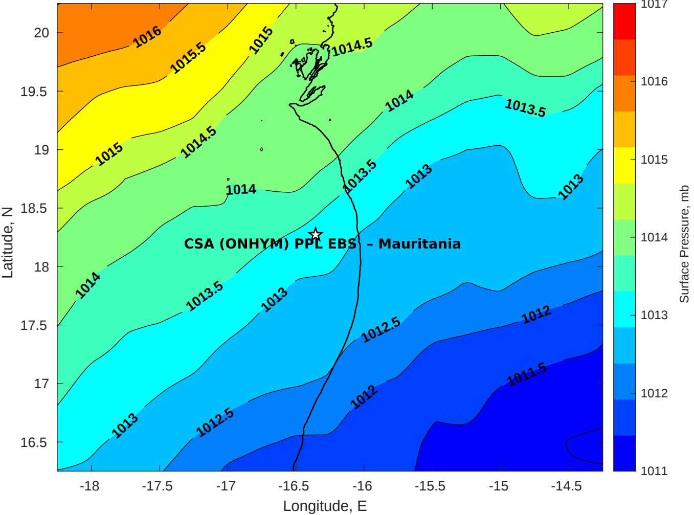
Surface Pressure (mb) for CSA (ONHYM) PPL EBS - Mauritania at 16-Nov-2025 00:00:00
